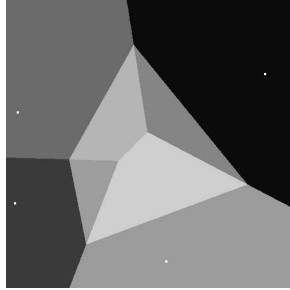
Figure 1: Area stolen when a query point is inserted into a Voronoi diagram.
