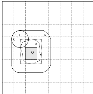
Figure 3: A uniform grid applied over the input domain. A is the axis-aligned bounding rectangle of the accumulative stolen area of a subdivision Q and R = A \oplus C where C is a square of edge-length 2l .
