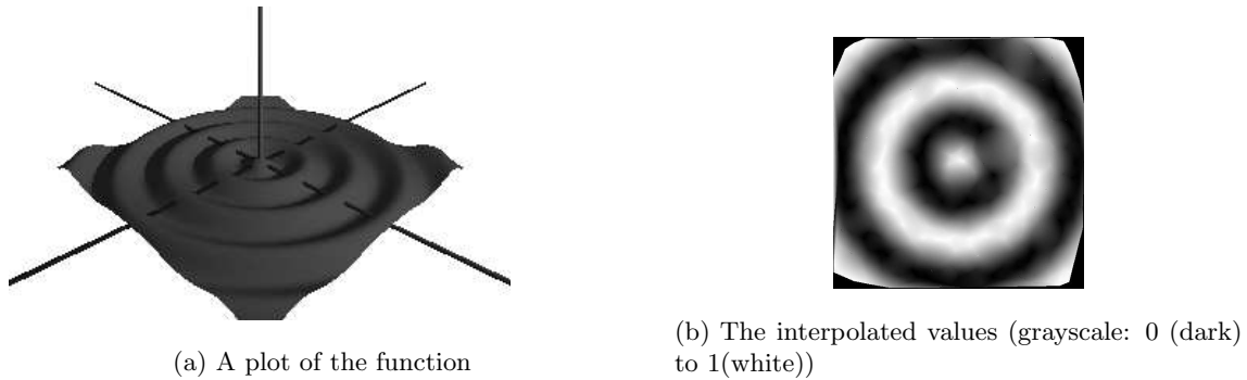
Figure 2: The scalar field generated by our algorithm
